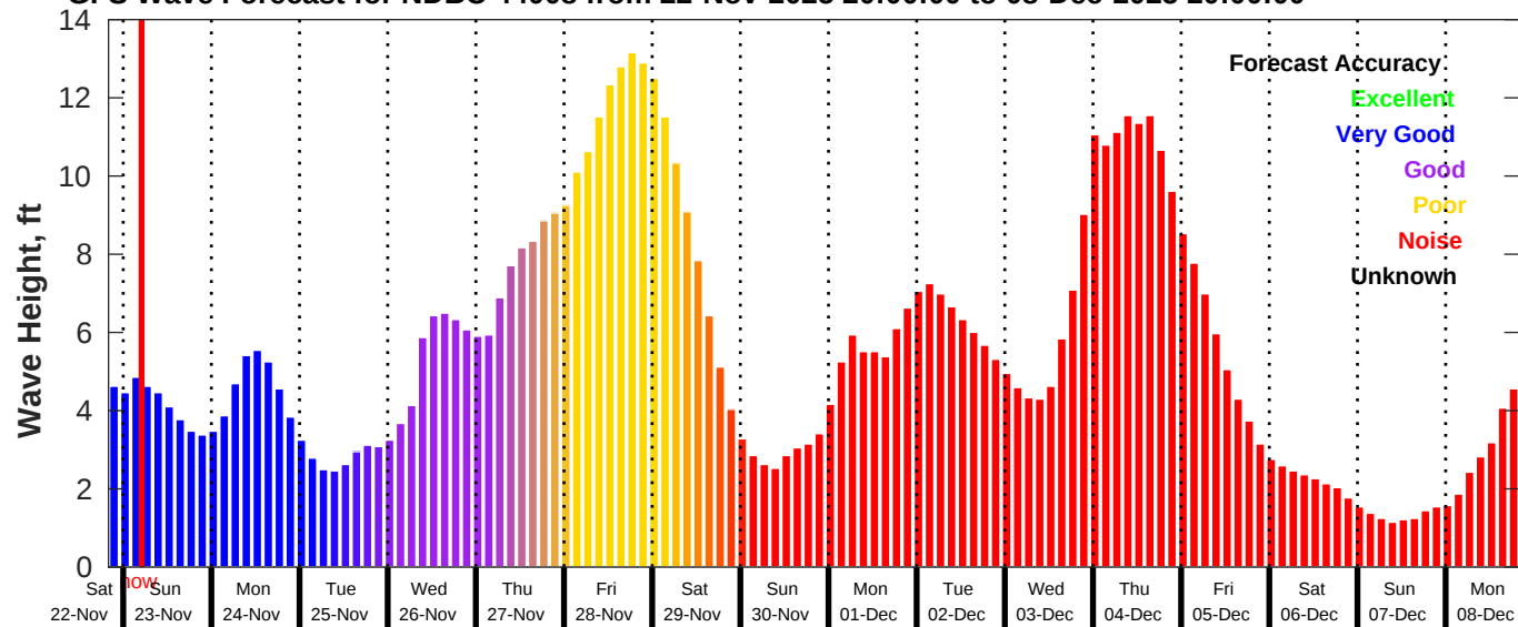
GFS Wave Forecast for NDBC 44008 from 22-Nov-2025 20:00:00 to 08-Dec-2025 20:00:00
