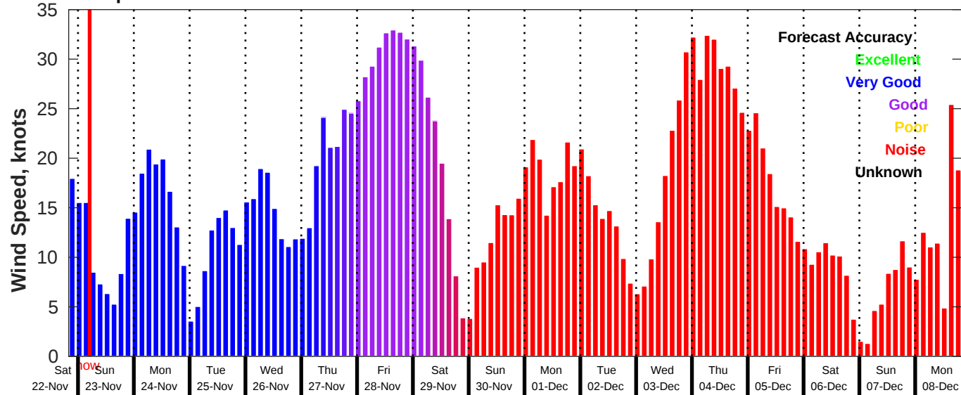
GFS Wind Speed Forecast for NDBC 44008 from 22-Nov-2025 20:00:00 to 08-Dec-2025 20:00:00
