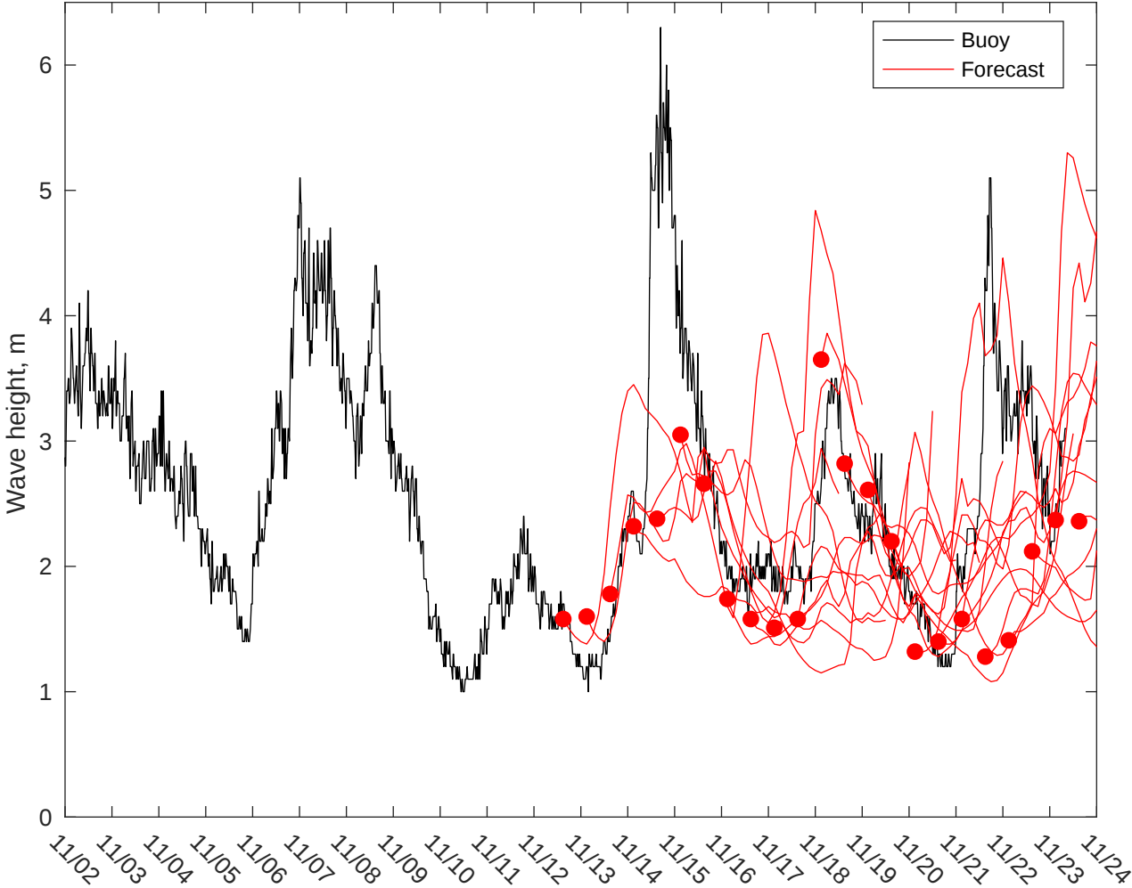
NDBC 46011 vs GFS Waves: 10 to 16 day forecast
