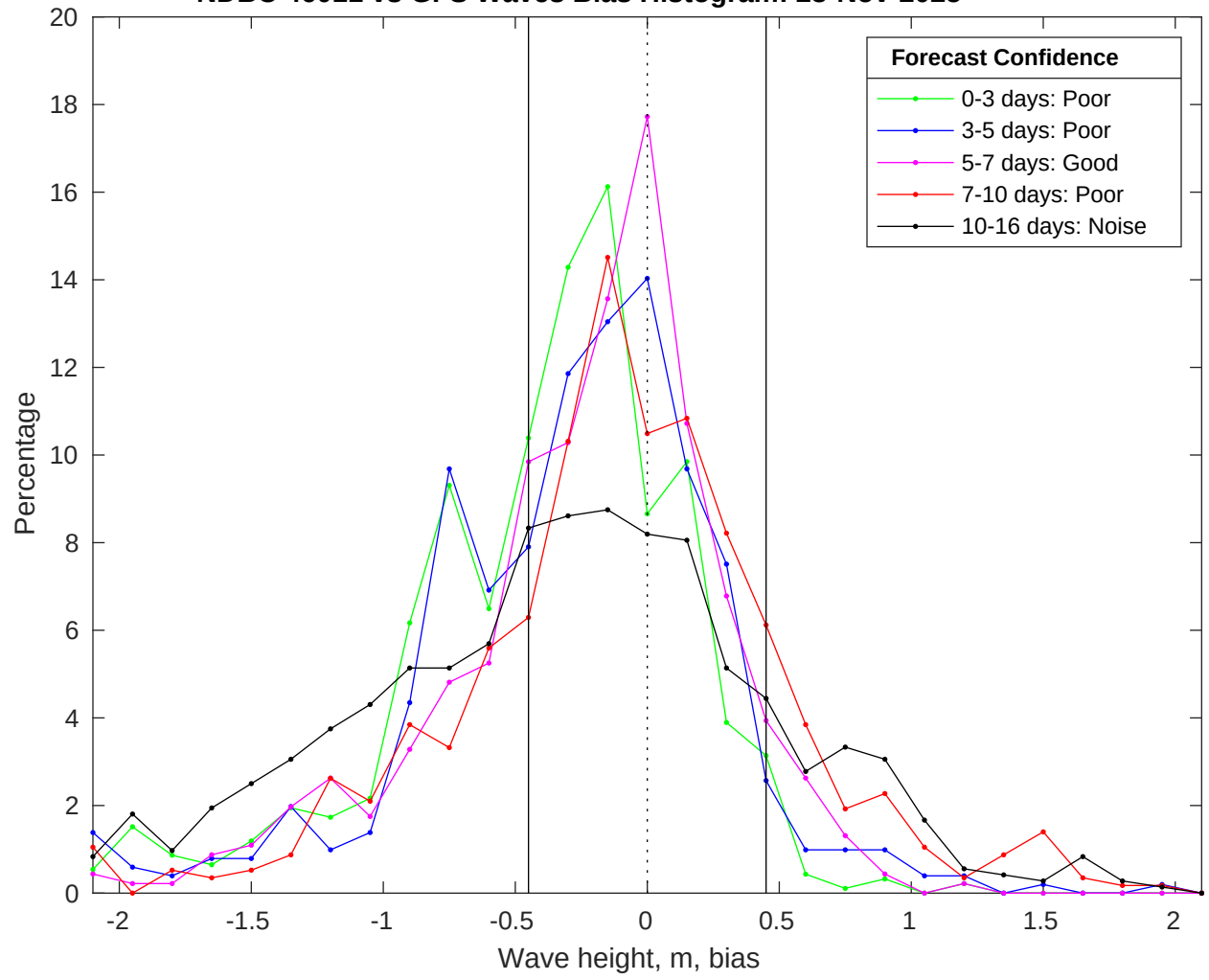
NDBC 46011 vs GFS Waves Bias Histogram: 23-Nov-2025
