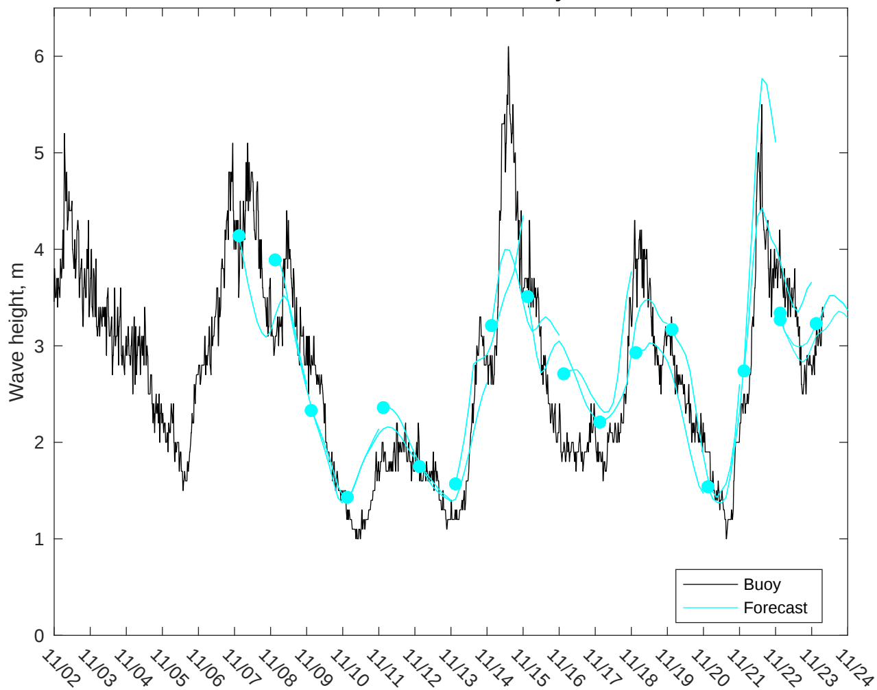
NDBC 46028 vs CMEMS Waves: 5 to 7 day forecast
