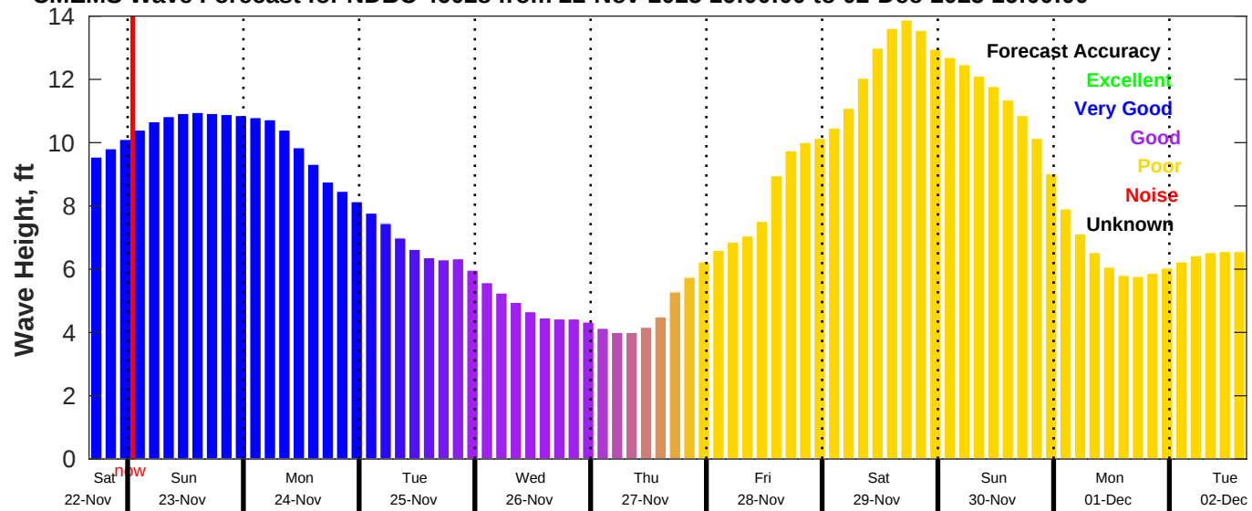
CMEMS Wave Forecast for NDBC 46028 from 22-Nov-2025 16:00:00 to 02-Dec-2025 16:00:00
