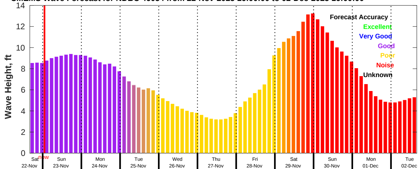
CMEMS Wave Forecast for NDBC 46054 from 22-Nov-2025 16:00:00 to 02-Dec-2025 16:00:00
