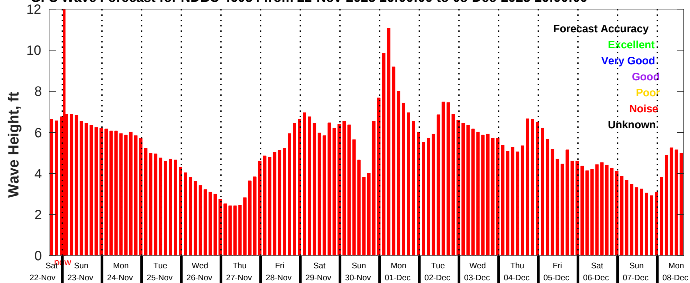
GFS Wave Forecast for NDBC 46054 from 22-Nov-2025 16:00:00 to 08-Dec-2025 16:00:00
