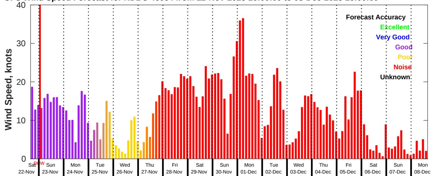
GFS Wind Speed Forecast for NDBC 46054 from 22-Nov-2025 16:00:00 to 08-Dec-2025 16:00:00
