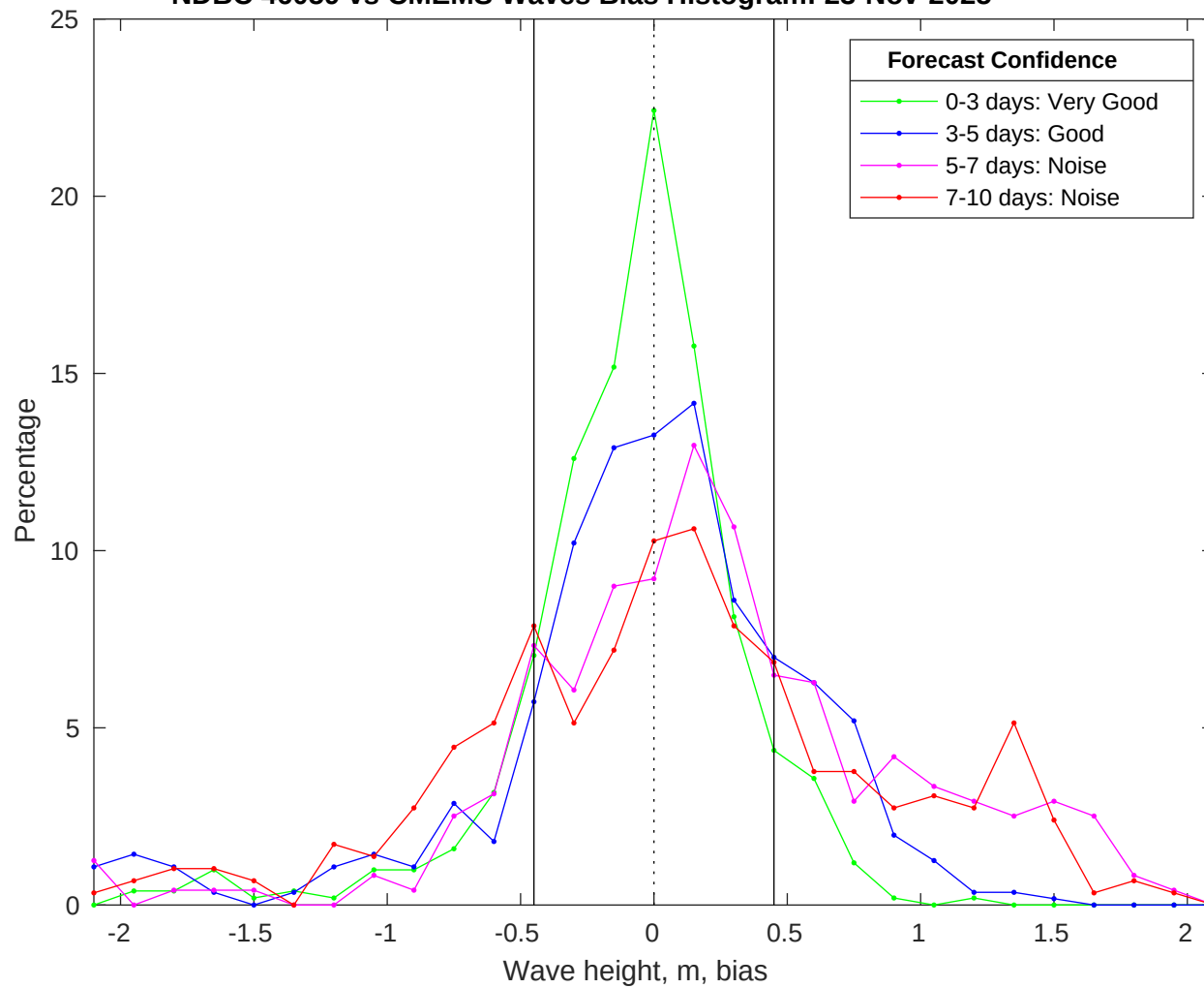
NDBC 46059 vs CMEMS Waves Bias Histogram: 23-Nov-2025
