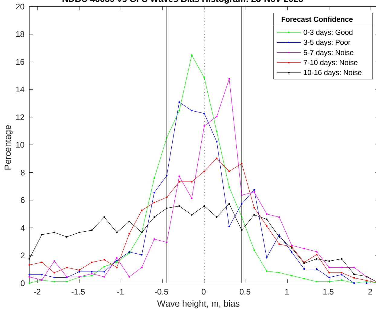
NDBC 46059 vs GFS Waves Bias Histogram: 23-Nov-2025
