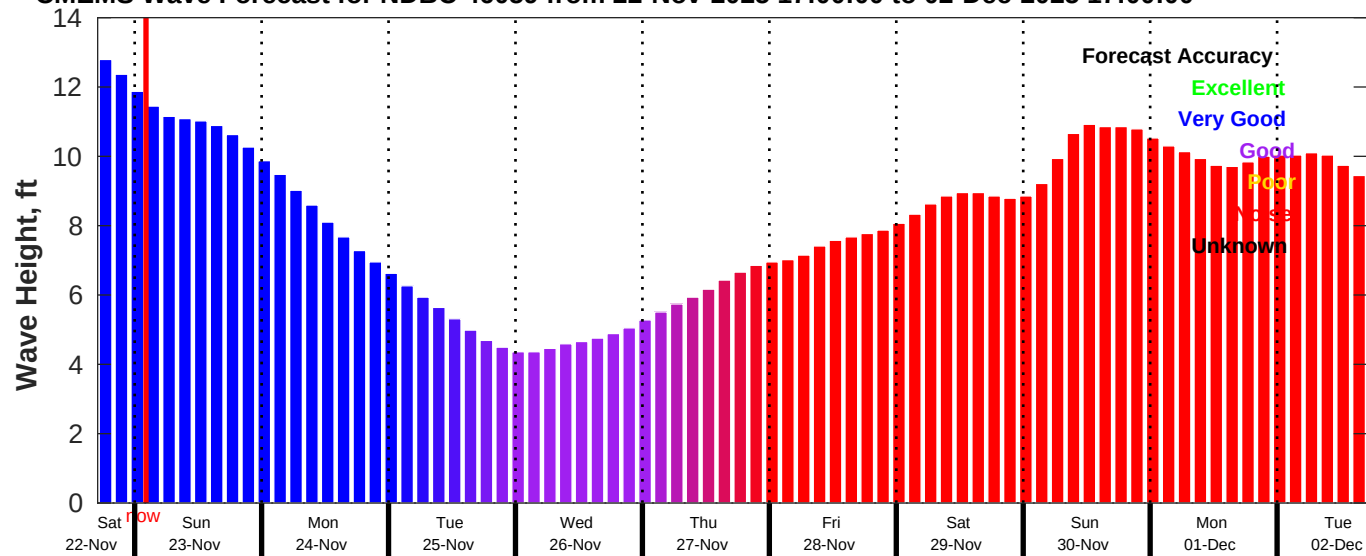
CMEMS Wave Forecast for NDBC 46059 from 22-Nov-2025 17:00:00 to 02-Dec-2025 17:00:00
