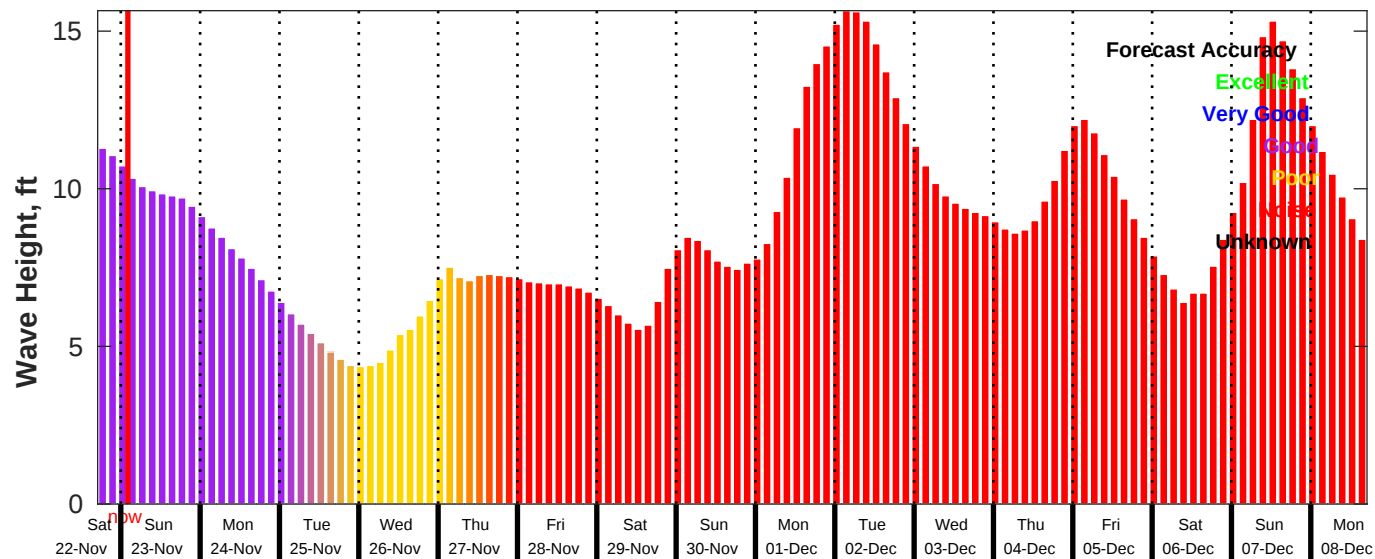
GFS Wave Forecast for NDBC 46059 from 22-Nov-2025 17:00:00 to 08-Dec-2025 17:00:00
