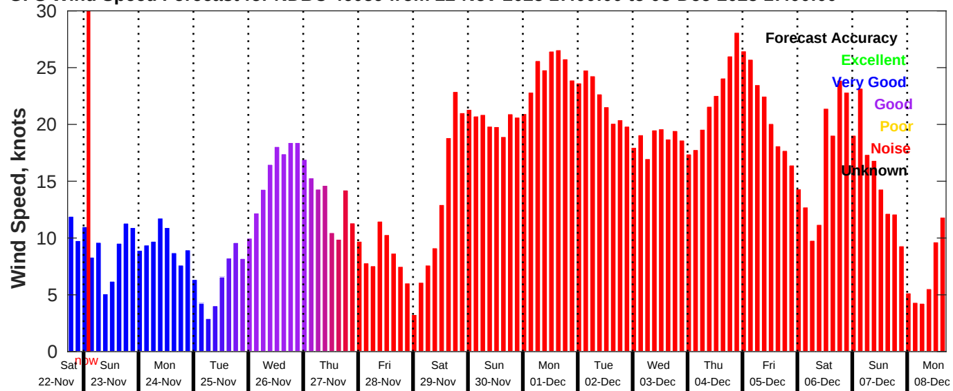
GFS Wind Speed Forecast for NDBC 46059 from 22-Nov-2025 17:00:00 to 08-Dec-2025 17:00:00
