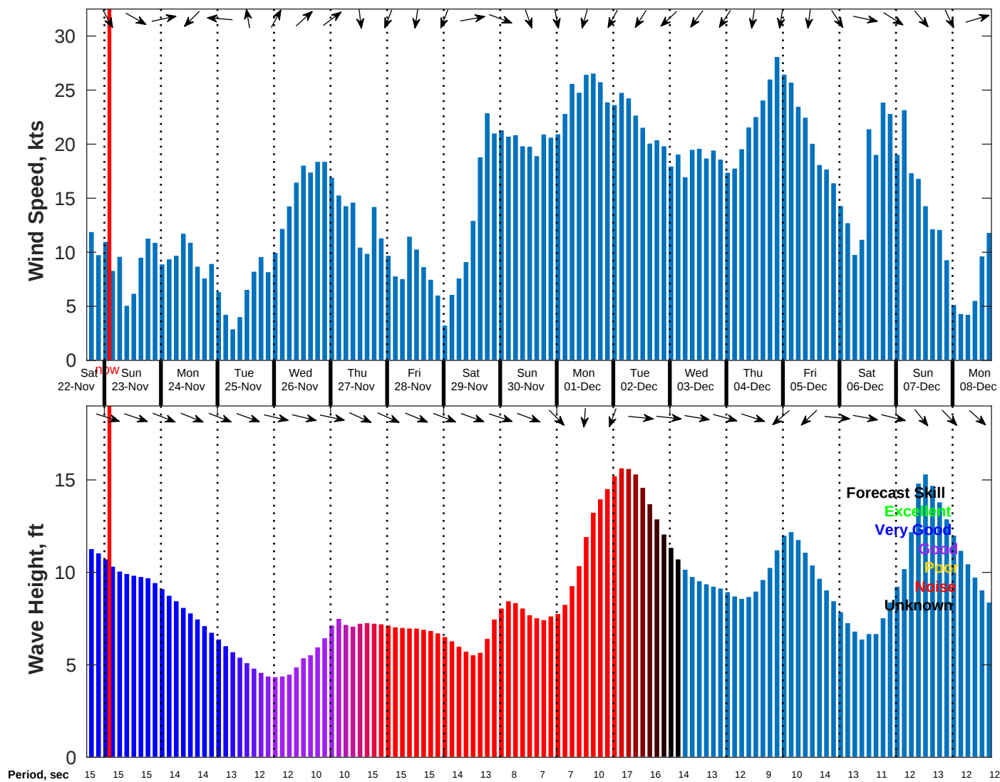
Wind & Wave Forecast for NDBC 46059 from 22-Nov-2025 17:00:00 to 08-Dec-2025 17:00:00
