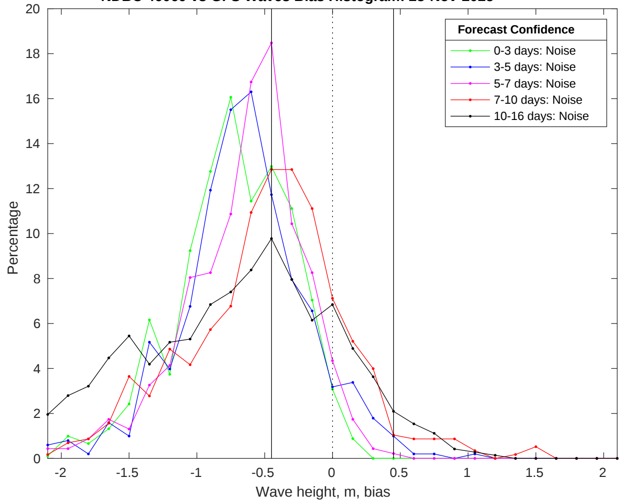
NDBC 46069 vs GFS Waves Bias Histogram: 23-Nov-2025
