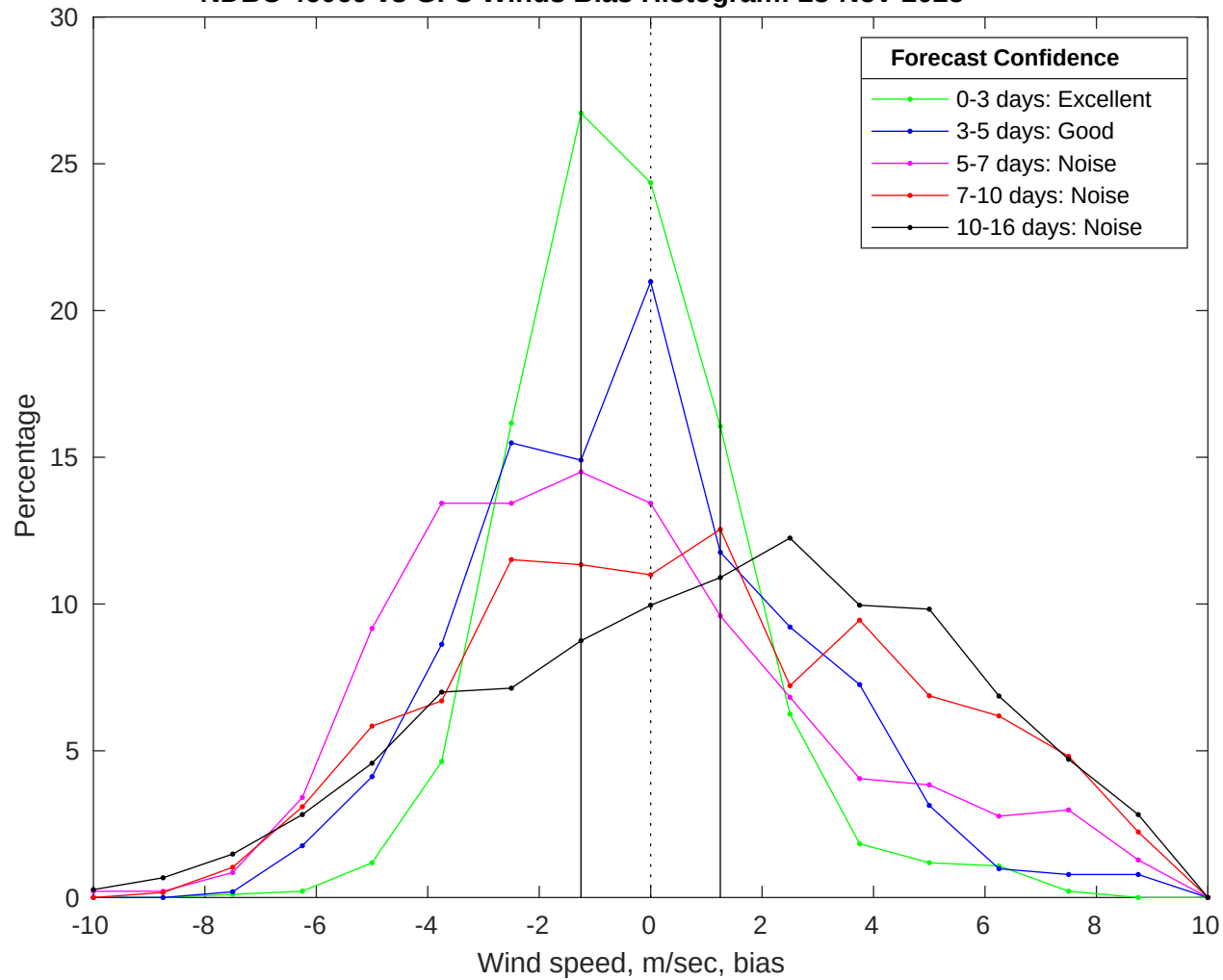
NDBC 46069 vs GFS Winds Bias Histogram: 23-Nov-2025
