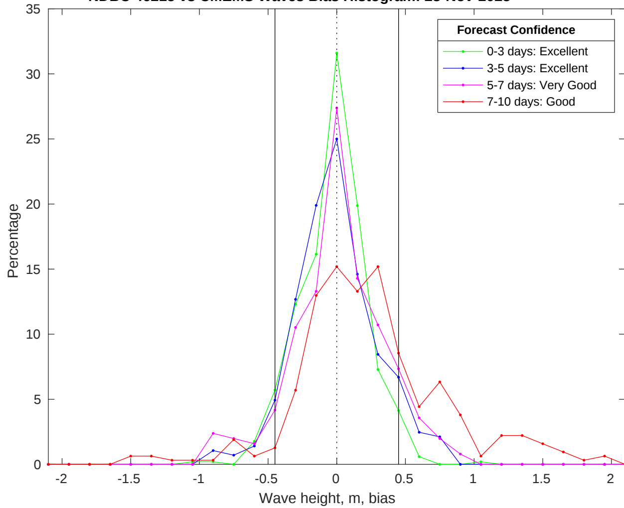
NDBC 46215 vs CMEMS Waves Bias Histogram: 23-Nov-2025
