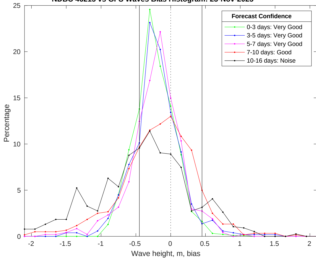
NDBC 46215 vs GFS Waves Bias Histogram: 23-Nov-2025
