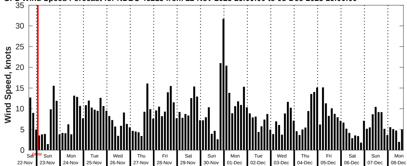
GFS Wind Speed Forecast for NDBC 46215 from 22-Nov-2025 16:00:00 to 08-Dec-2025 16:00:00
