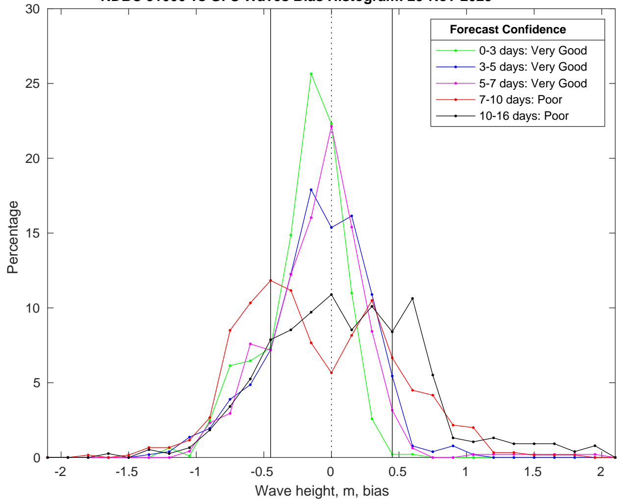
NDBC 51000 vs GFS Waves Bias Histogram: 23-Nov-2025
