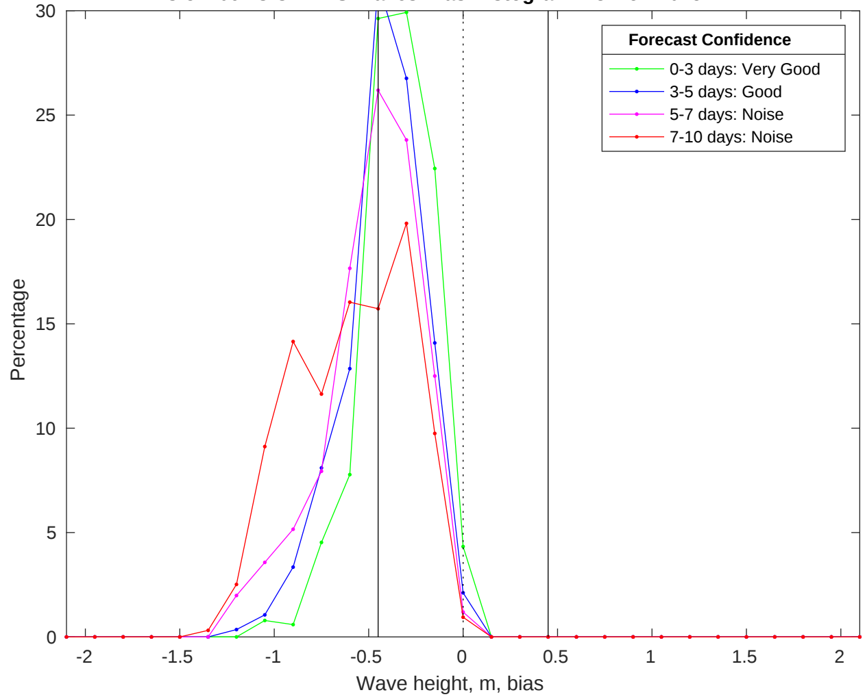
NDBC 51209 vs CMEMS Waves Bias Histogram: 23-Nov-2025
