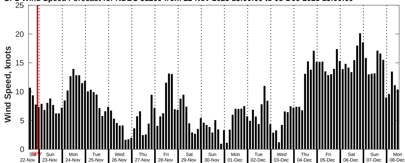
GFS Wind Speed Forecast for NDBC 51209 from 22-Nov-2025 13:00:00 to 08-Dec-2025 13:00:00
