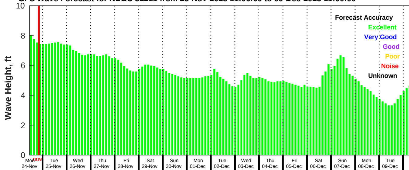
GFS Wave Forecast for NDBC 52211 from 23-Nov-2025 11:00:00 to 09-Dec-2025 11:00:00
