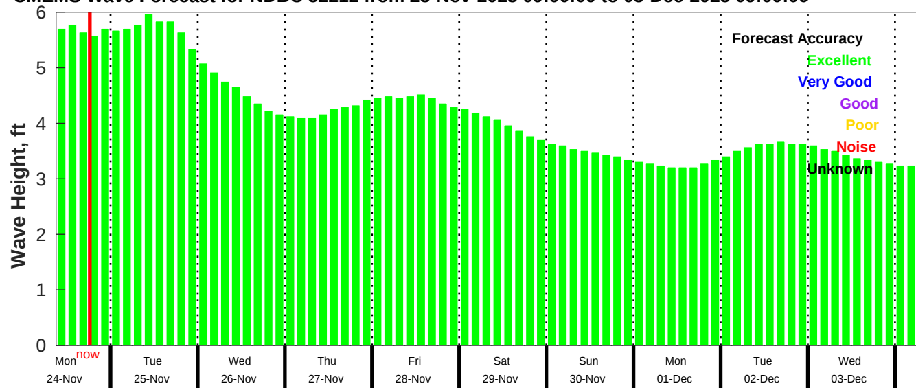
CMEMS Wave Forecast for NDBC 52212 from 23-Nov-2025 09:00:00 to 03-Dec-2025 09:00:00
