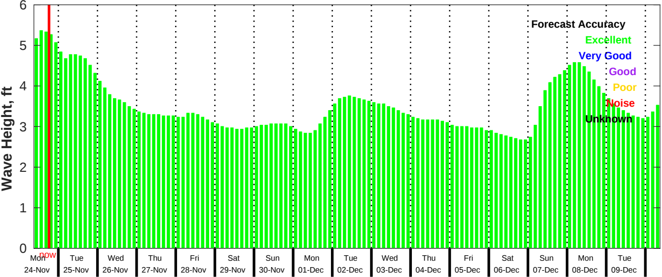
GFS Wave Forecast for NDBC 52212 from 23-Nov-2025 09:00:00 to 09-Dec-2025 09:00:00
