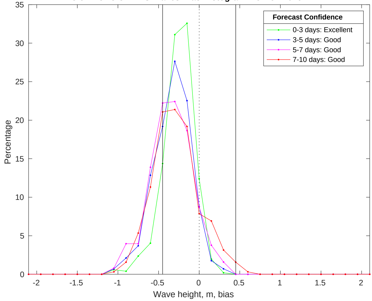
NDBC 52213 vs CMEMS Waves Bias Histogram: 23-Nov-2025
