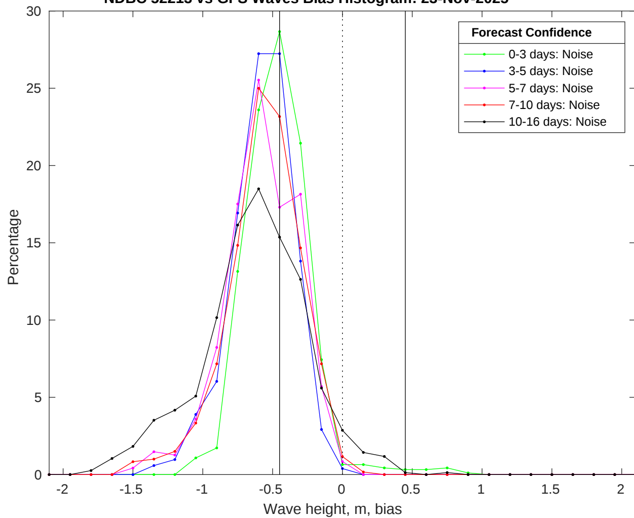
NDBC 52213 vs GFS Waves Bias Histogram: 23-Nov-2025
