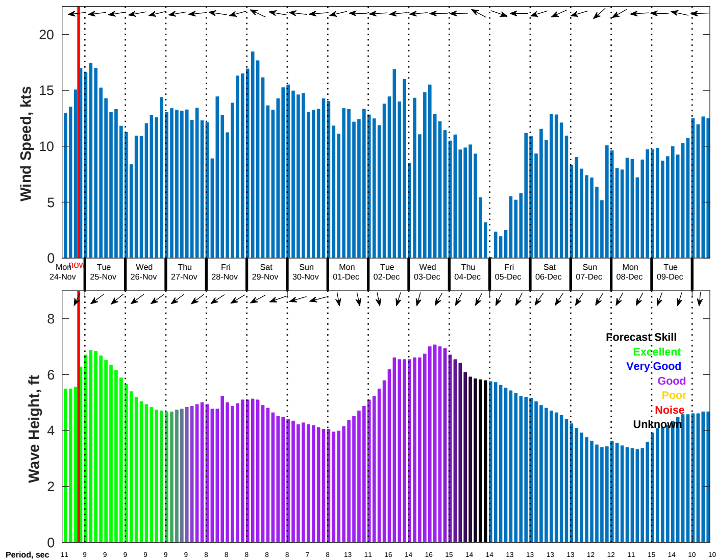
Wind & Wave Forecast for NDBC 52213 from 23-Nov-2025 11:00:00 to 09-Dec-2025 11:00:00
