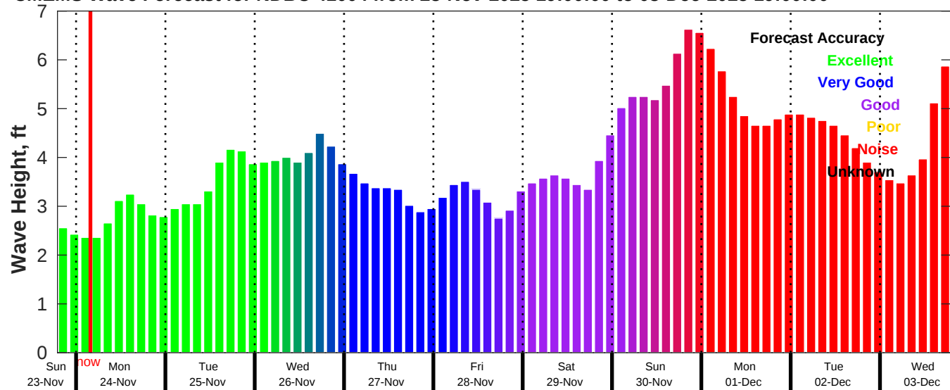
CMEMS Wave Forecast for NDBC 41004 from 23-Nov-2025 19:00:00 to 03-Dec-2025 19:00:00
