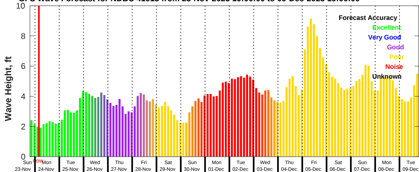
GFS Wave Forecast for NDBC 41013 from 23-Nov-2025 19:00:00 to 09-Dec-2025 19:00:00
