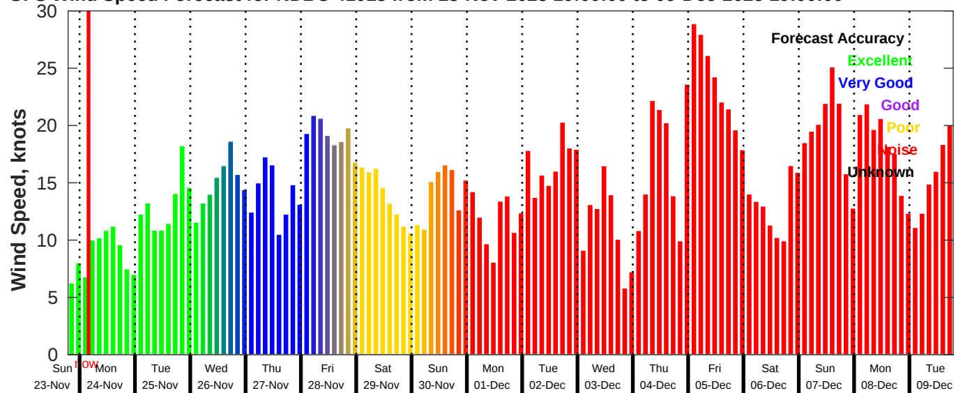
GFS Wind Speed Forecast for NDBC 41013 from 23-Nov-2025 19:00:00 to 09-Dec-2025 19:00:00
