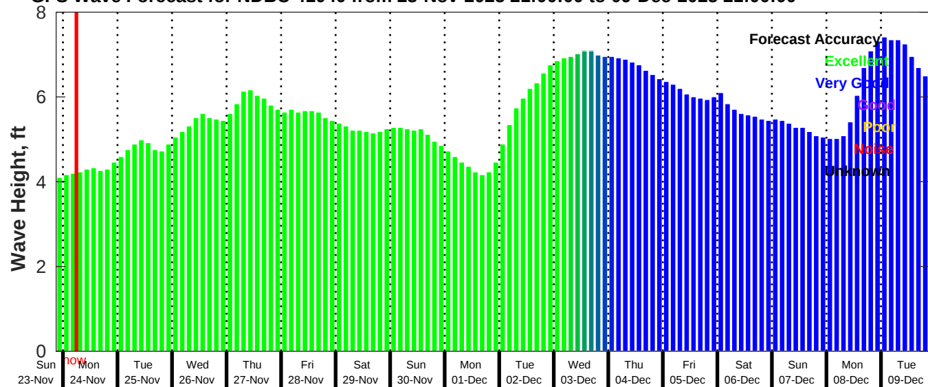
GFS Wave Forecast for NDBC 41040 from 23-Nov-2025 21:00:00 to 09-Dec-2025 21:00:00
