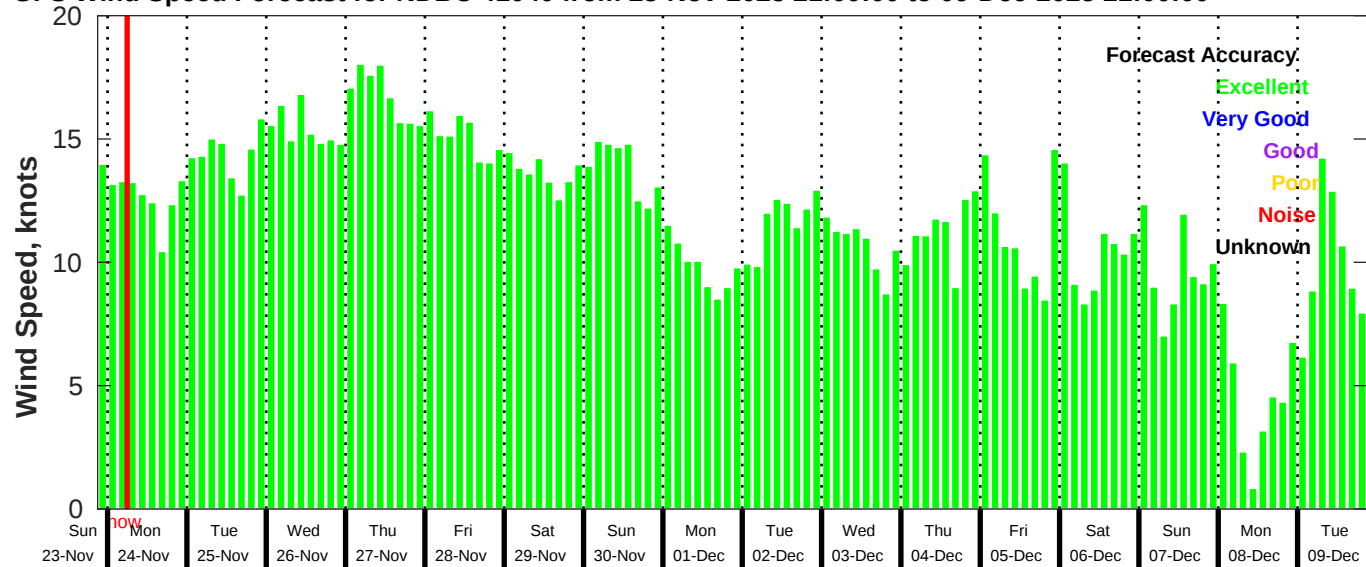
GFS Wind Speed Forecast for NDBC 41040 from 23-Nov-2025 21:00:00 to 09-Dec-2025 21:00:00
