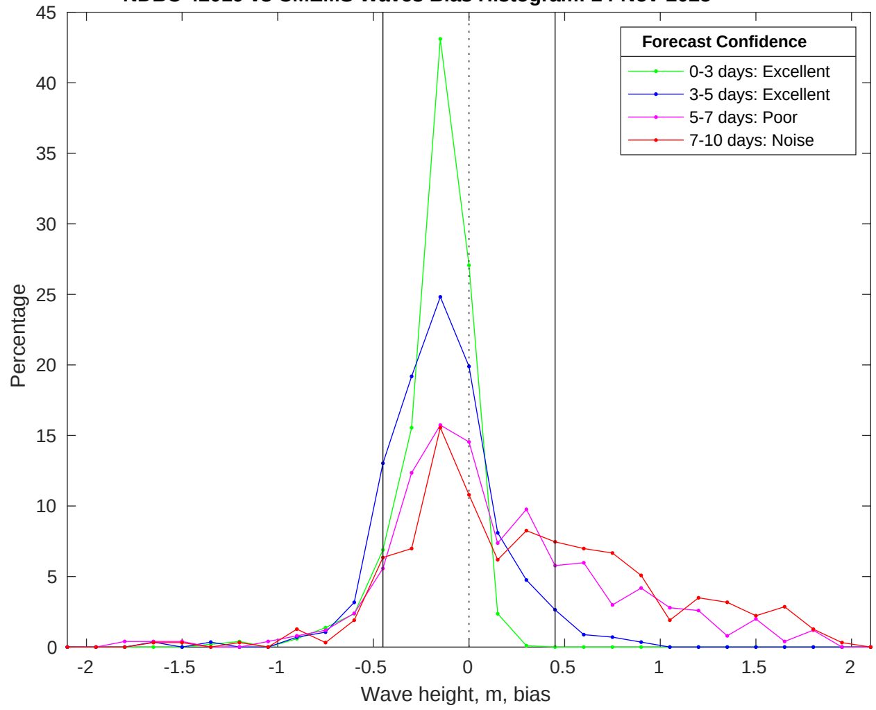
NDBC 42019 vs CMEMS Waves Bias Histogram: 24-Nov-2025
