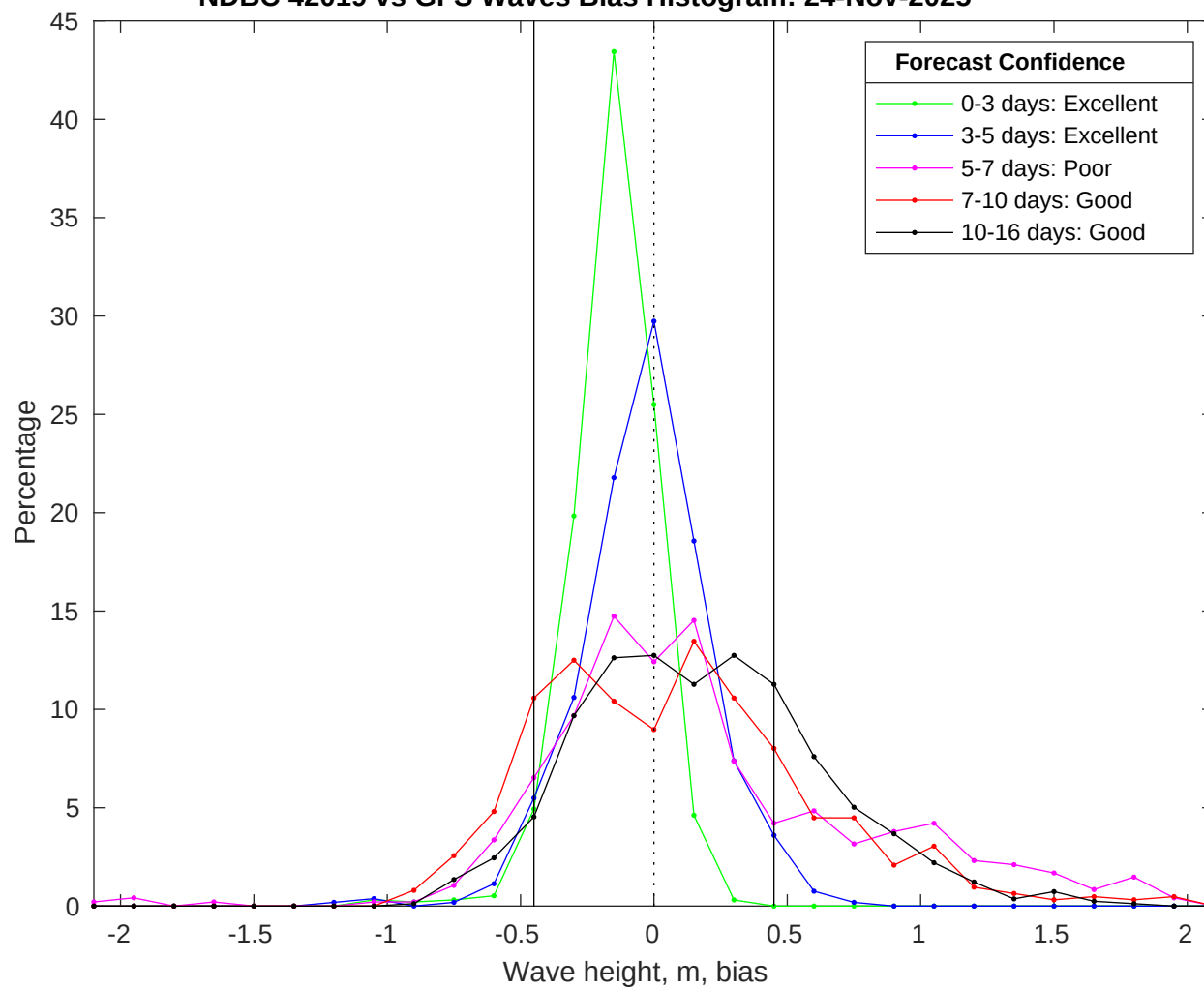
NDBC 42019 vs GFS Waves Bias Histogram: 24-Nov-2025
