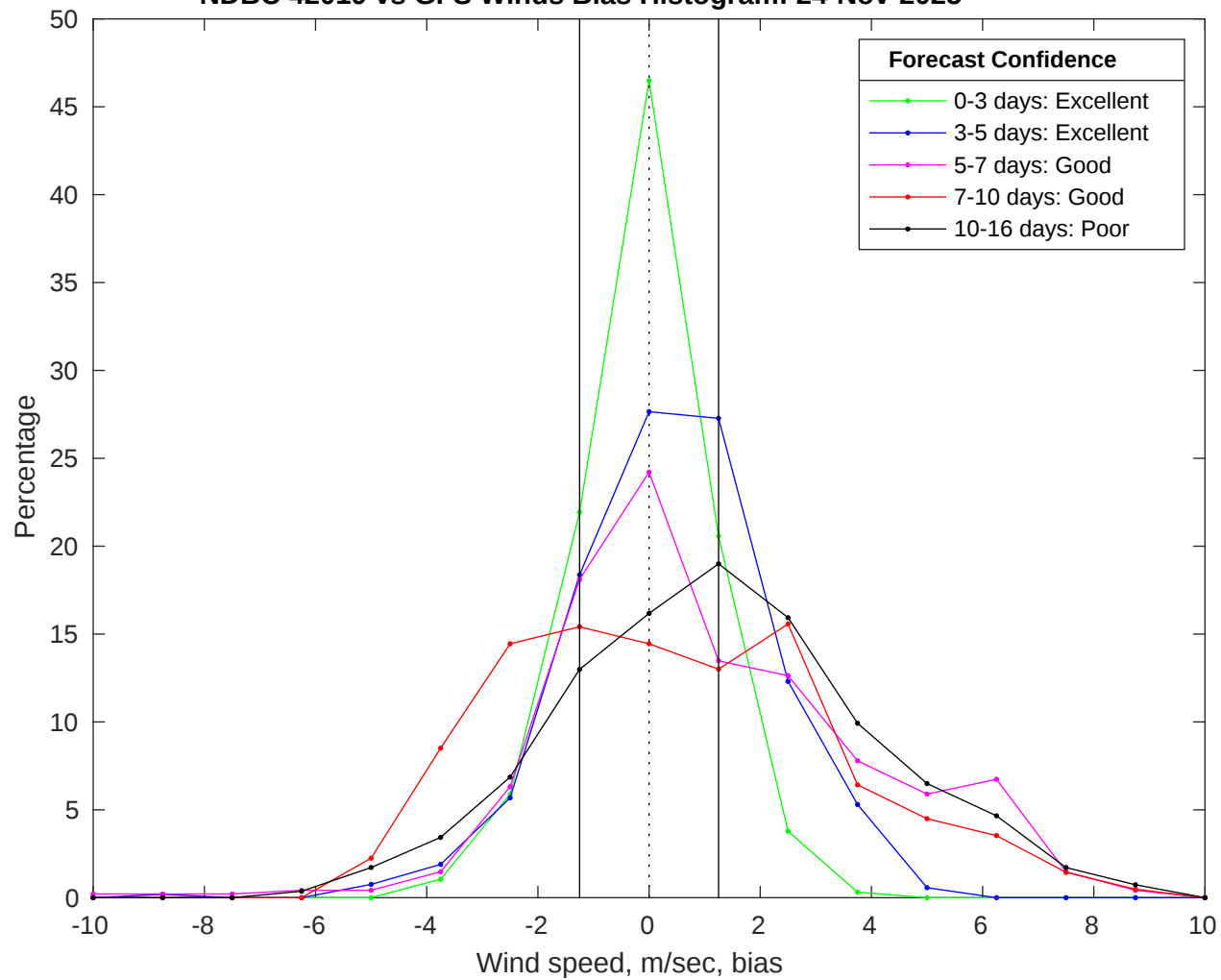
NDBC 42019 vs GFS Winds Bias Histogram: 24-Nov-2025
