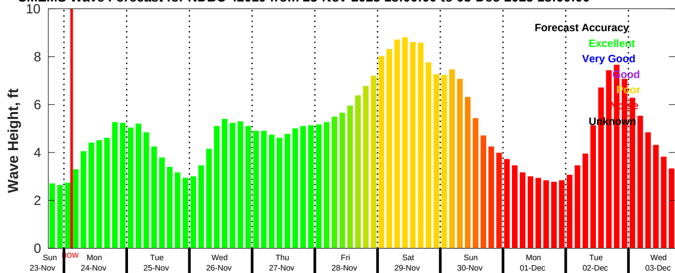
CMEMS Wave Forecast for NDBC 42019 from 23-Nov-2025 18:00:00 to 03-Dec-2025 18:00:00
