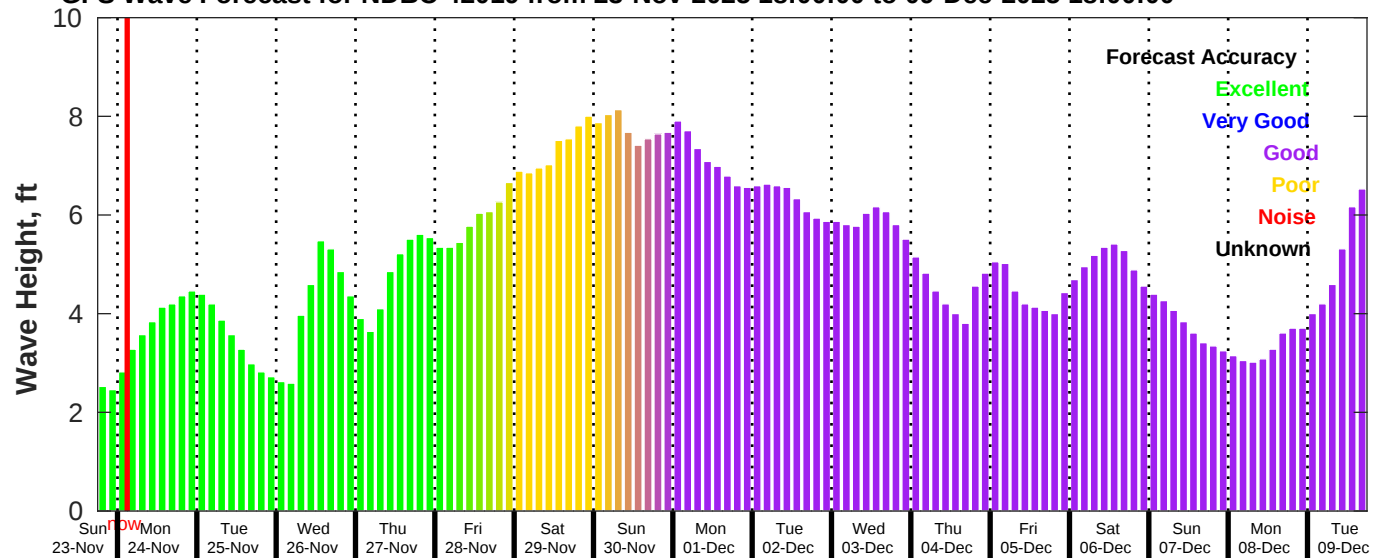
GFS Wave Forecast for NDBC 42019 from 23-Nov-2025 18:00:00 to 09-Dec-2025 18:00:00
