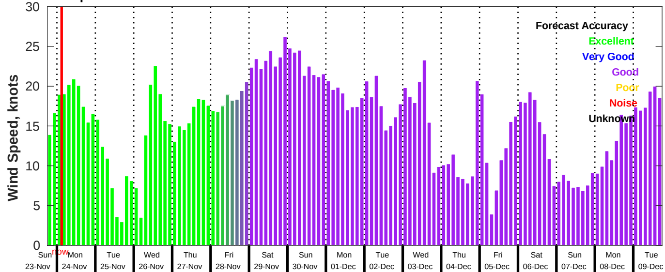
GFS Wind Speed Forecast for NDBC 42020 from 23-Nov-2025 18:00:00 to 09-Dec-2025 18:00:00
