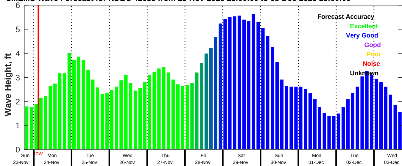
CMEMS Wave Forecast for NDBC 42035 from 23-Nov-2025 18:00:00 to 03-Dec-2025 18:00:00
