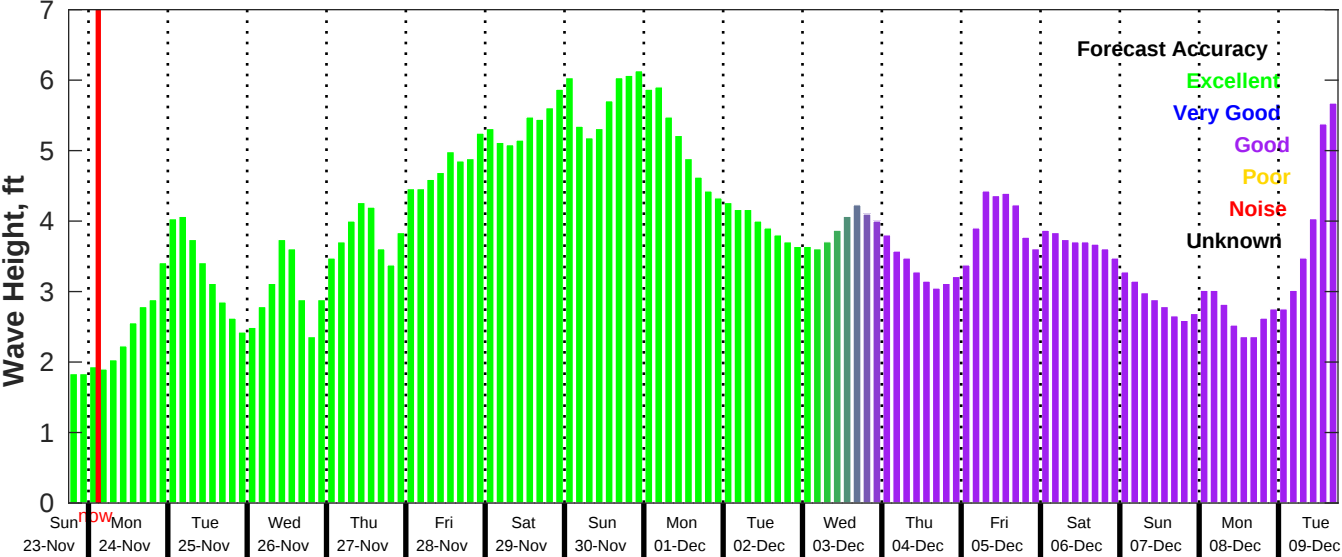
GFS Wave Forecast for NDBC 42035 from 23-Nov-2025 18:00:00 to 09-Dec-2025 18:00:00
