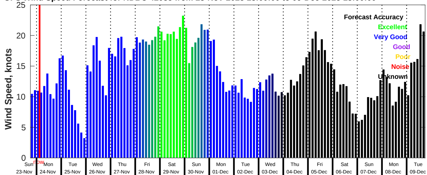
GFS Wind Speed Forecast for NDBC 42035 from 23-Nov-2025 18:00:00 to 09-Dec-2025 18:00:00
