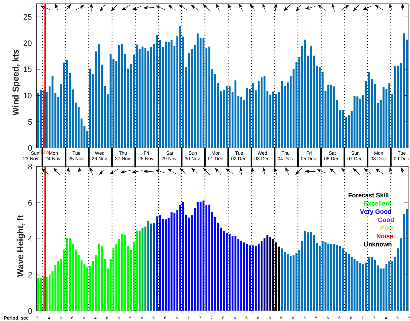
Wind & Wave Forecast for NDBC 42035 from 23-Nov-2025 18:00:00 to 09-Dec-2025 18:00:00
