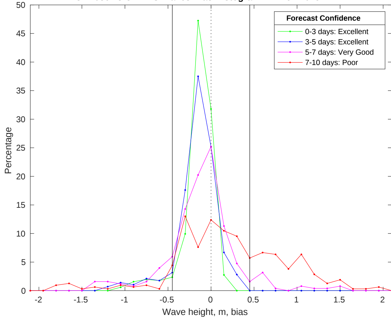
NDBC 42036 vs CMEMS Waves Bias Histogram: 24-Nov-2025
