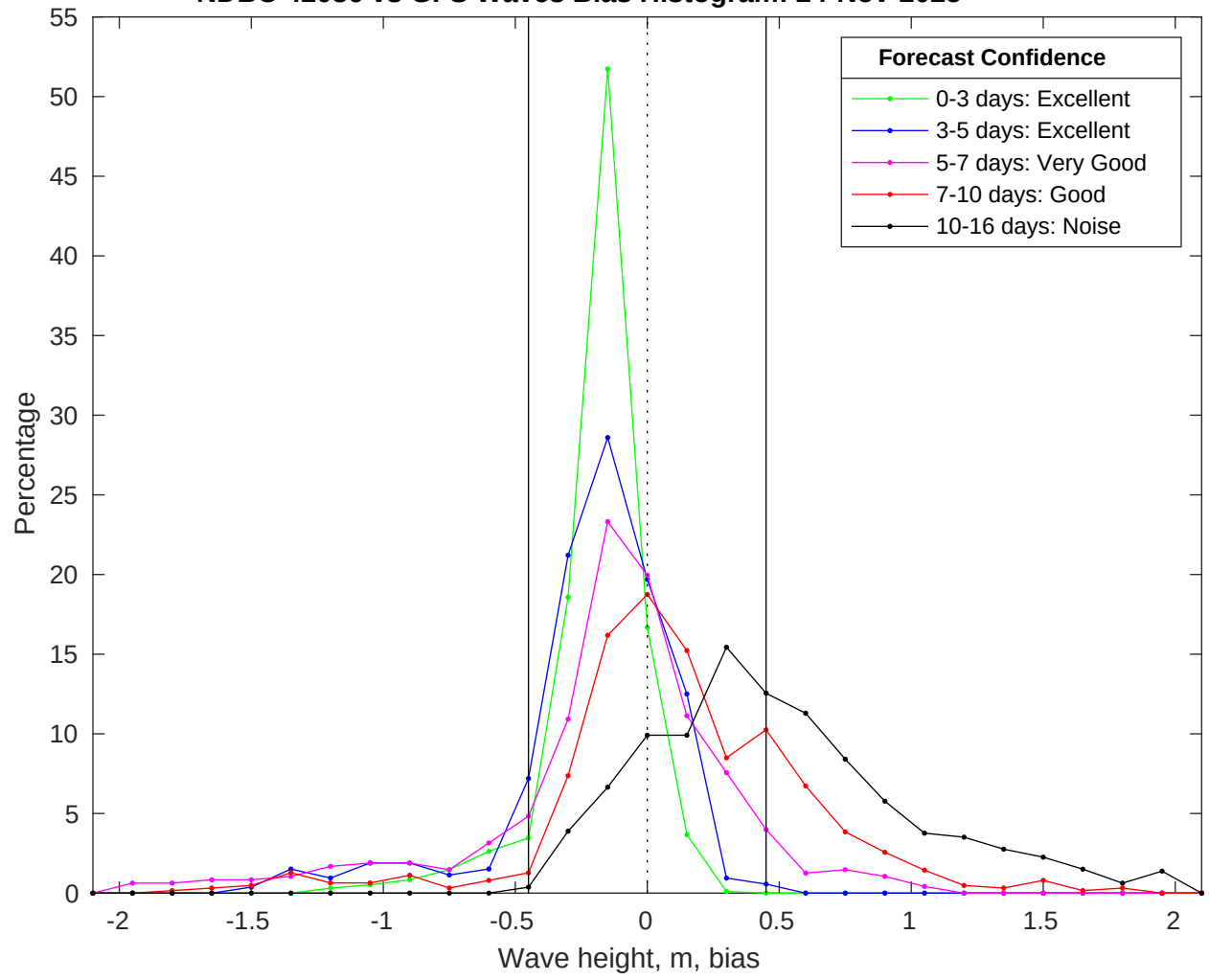
NDBC 42036 vs GFS Waves Bias Histogram: 24-Nov-2025
