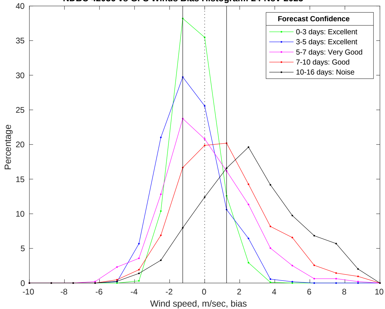
NDBC 42036 vs GFS Winds Bias Histogram: 24-Nov-2025
