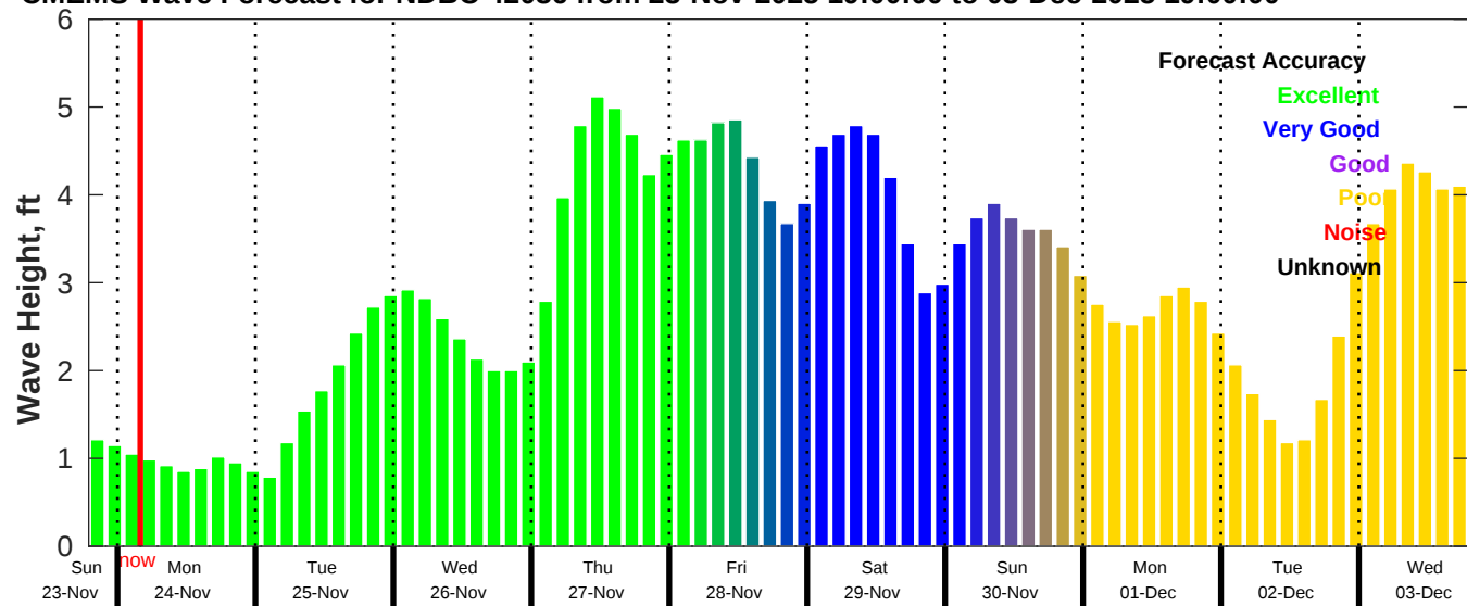
CMEMS Wave Forecast for NDBC 42036 from 23-Nov-2025 19:00:00 to 03-Dec-2025 19:00:00
