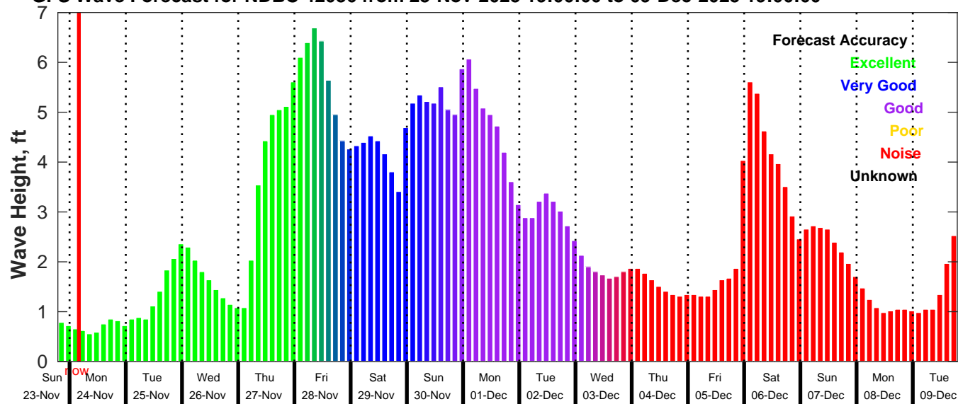
GFS Wave Forecast for NDBC 42036 from 23-Nov-2025 19:00:00 to 09-Dec-2025 19:00:00
