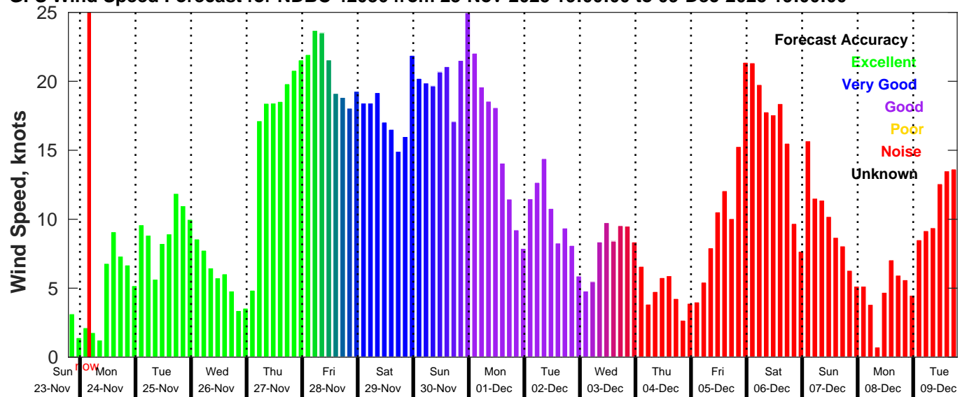
GFS Wind Speed Forecast for NDBC 42036 from 23-Nov-2025 19:00:00 to 09-Dec-2025 19:00:00
